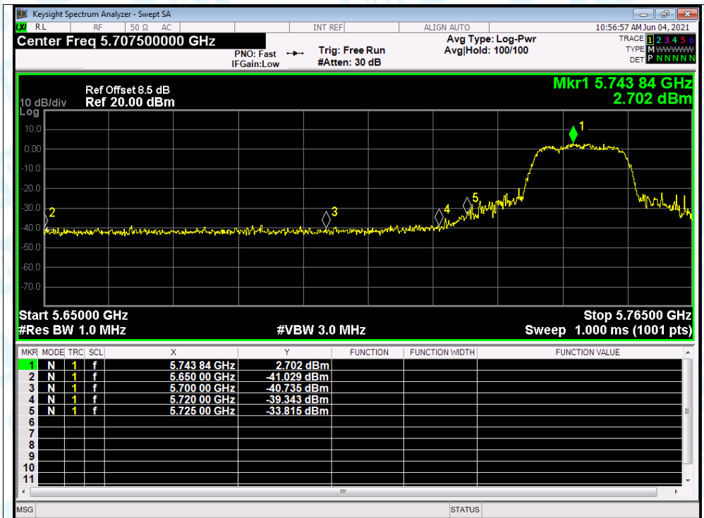
Restrict Band NVNT a 5745MHz Ant1 Average
