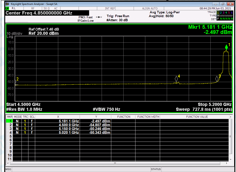
Restrict Band NVNT a 5180MHz Ant1 Average
