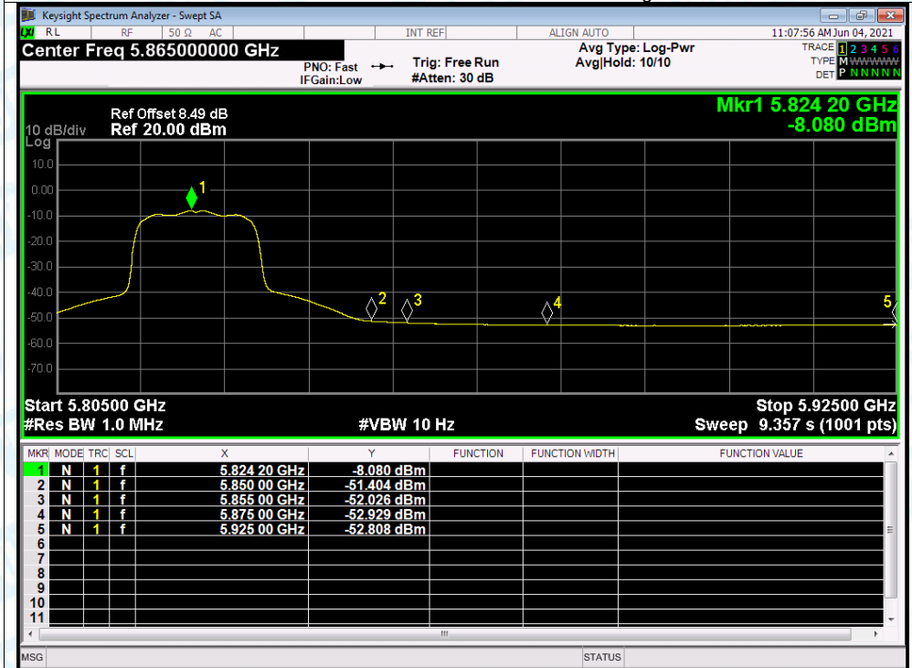
Restrict Band NVNT a 5825MHz Ant1 Average
