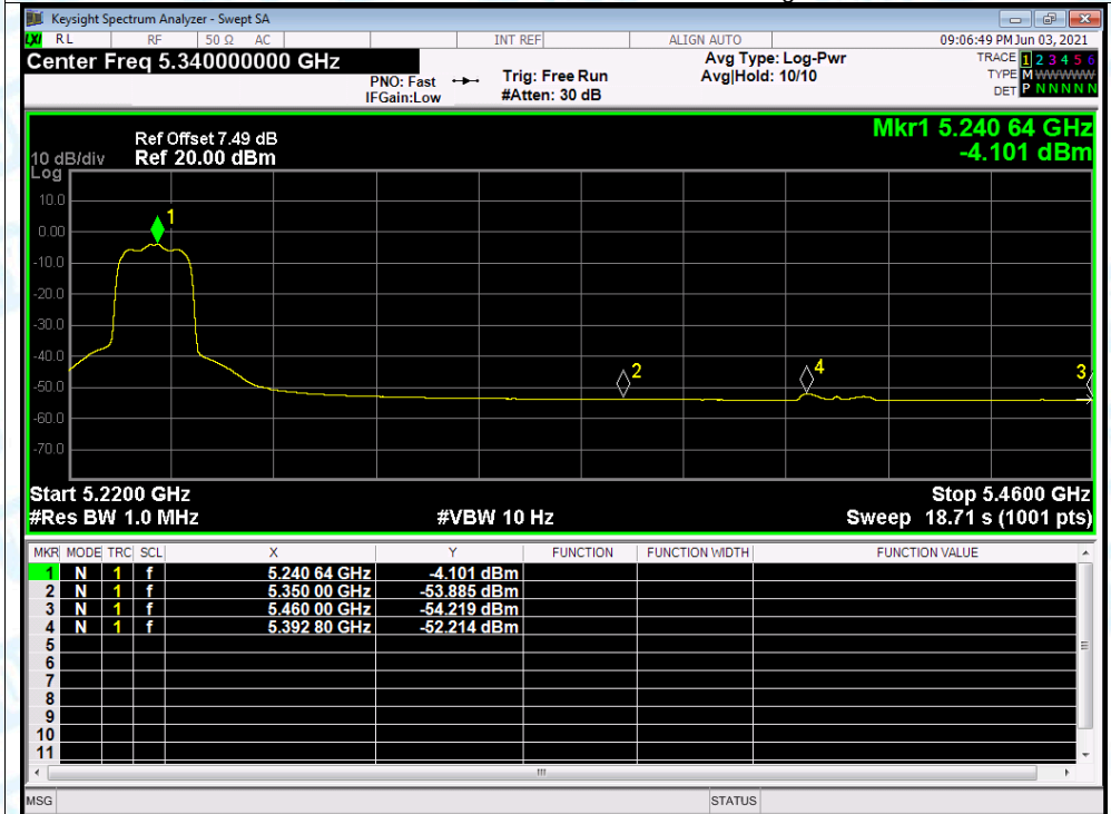
Restrict Band NVNT a 5240MHz Ant1 Average
